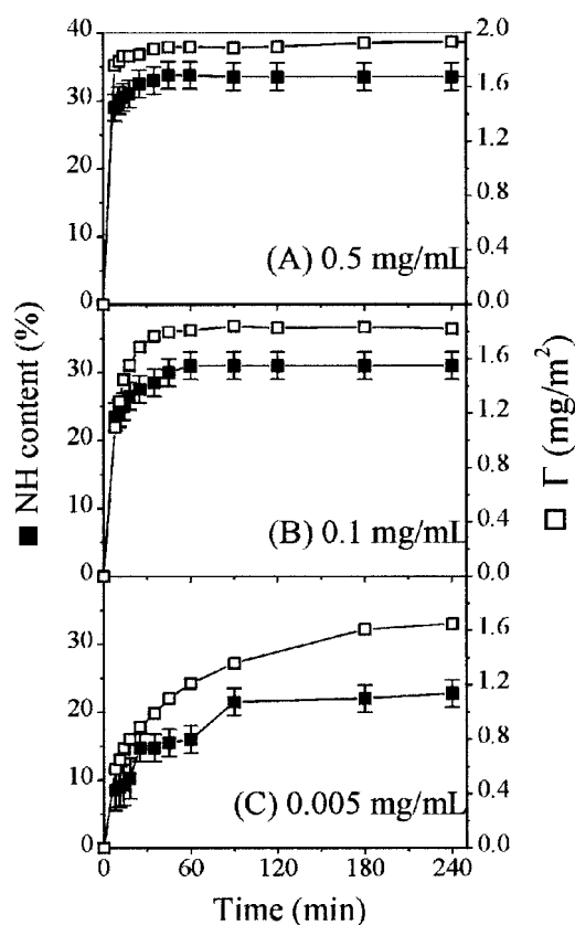
FIGURE 4 Changes in the residual amounts of peptide NH signal (in percentage of the overall peptide carbonyls) (■) and of the surface density \Gamma (□) with time for HLL adsorbed onto the hydrophobic surface at pH 7.5, at bulk concentrations of 0.5 mg/mL (A), 0.1 mg/mL (B), and 0.005 mg/mL (C).
